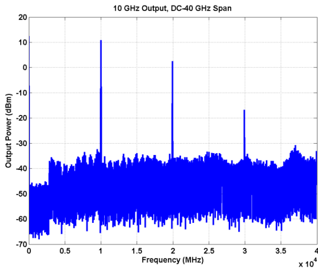
Figure 6 – 10 GHz Output, DC-40 GHz, VBW/RBW = 100 kHz
