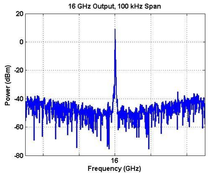
Figure 5 – 16 GHz Output, 100 kHz span, RBW = 100 Hz, VBW = 30 Hz
