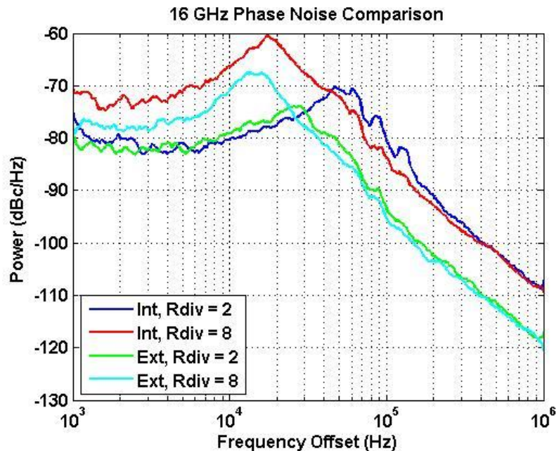
Figure 3 - Phase Noise Reference and Reference Divider Comparison
