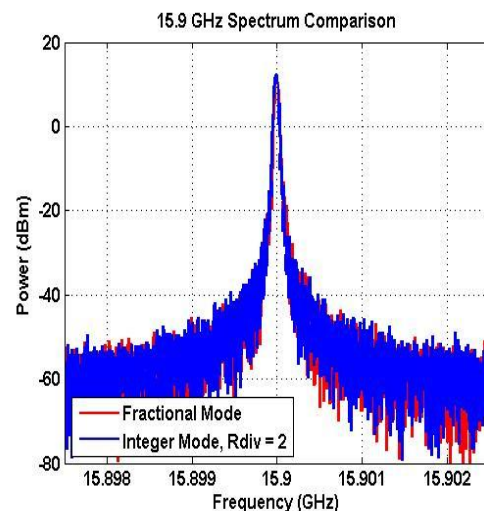
Figure 2 – Fractional vs. Integer Mode Spectrum 10 MHz span, RBW = 10 kHz, VBW = 300 Hz
