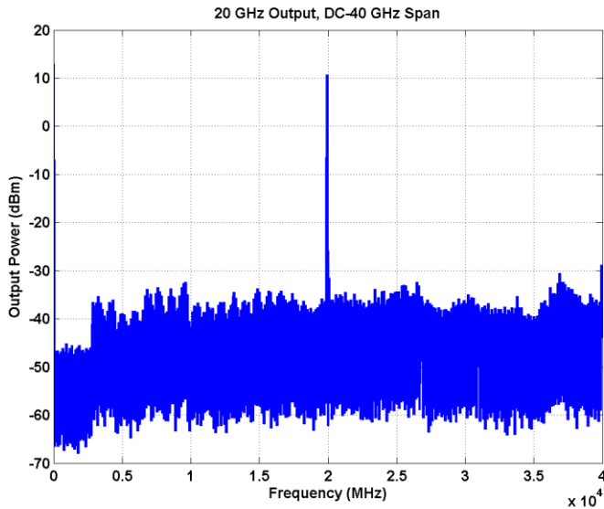
Figure 8 – 20 GHz Output, DC-40 GHz, VBW/RBW = 100 kHz
