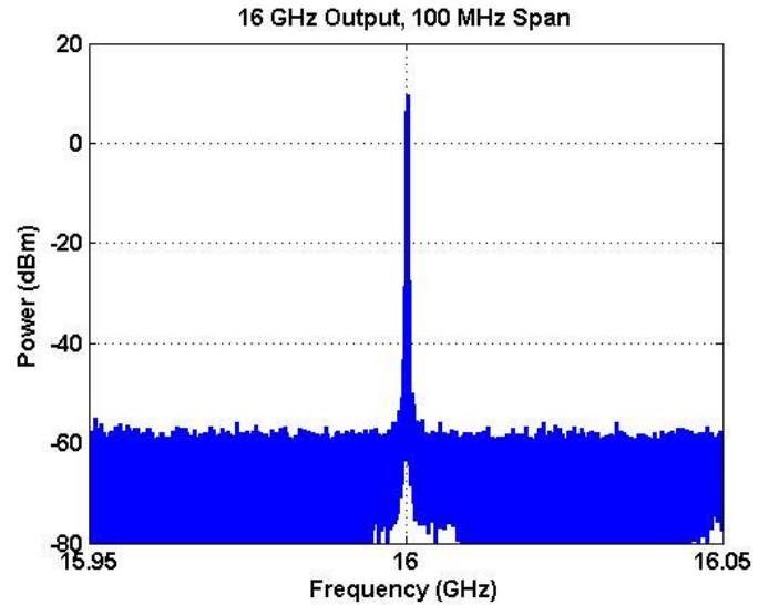
Figure 9 – 16 GHz Output, 100 MHz span, RBW = 10 kHz, VBW = 3 kHz
