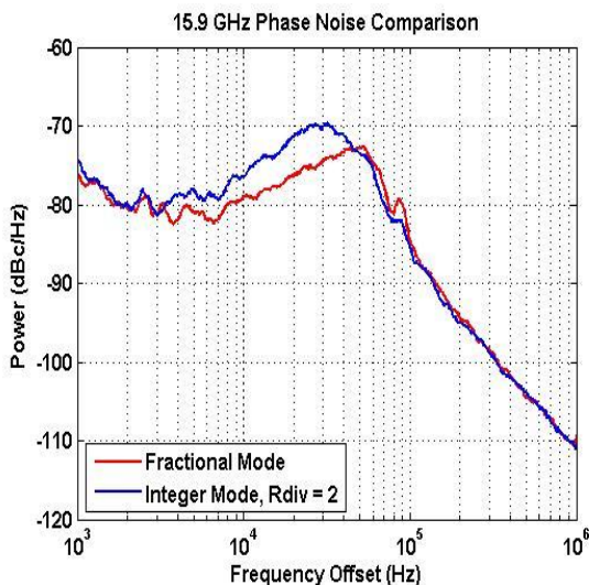
Figure 1 - Fractional vs. Integer Mode Phase Noise
