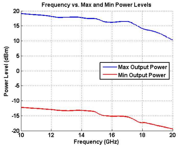
Figure 5 - Frequency vs. Output Power from 10 GHz to 20 GHz in 40 MHz steps
