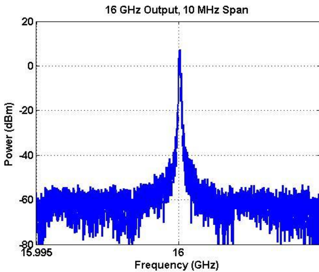
Figure 4 – 16 GHz Output, 10 MHz span, RBW = 3 kHz, VBW = 1 kHz
