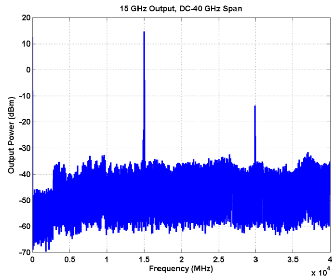
Figure 7 – 15 GHz Output, DC-40 GHz, VBW/RBW = 100 kHz
