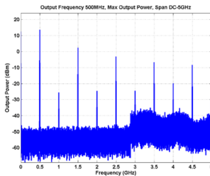
Figure 6 a),b),c) – Output Frequency 500 MHz, Span of 20 MHz, 5 GHz, 10 GHz
