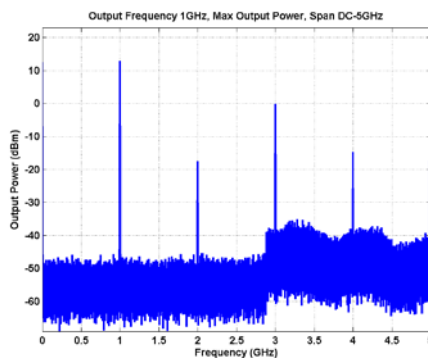
Figure 7 a),b),c) – Output Frequency 1 GHz, Span of 20 MHz, 5 GHz, 10 GHz
