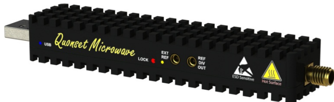
QM2010-6000 Side View USB, Lock Status, and External Reference LEDs External Reference MMCX input, Reference Out MMCX output
