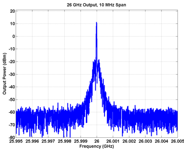
Figure 10 – 26 GHz Output, 10 MHz, RBW = 10 kHz, VBW = 1 kHz
