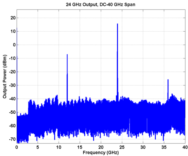
Figure 6 – 24 GHz Output, DC-40 GHz, RBW = 1 MHz, VBW = 10 kHz
