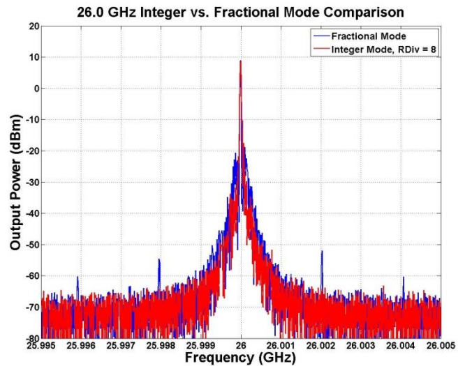
Figure 2 - Fractional vs. Integer Mode Mode Spectrum 10 MHz span, RBW = 10kHz, VBW = 300 Hz
