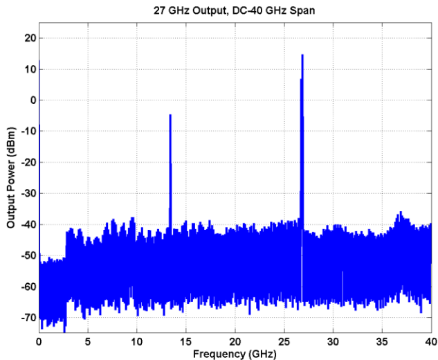
Figure 8 – 27 GHz Output, DC-40 GHz, RBW = 1 MHz, VBW = 10 kHz
