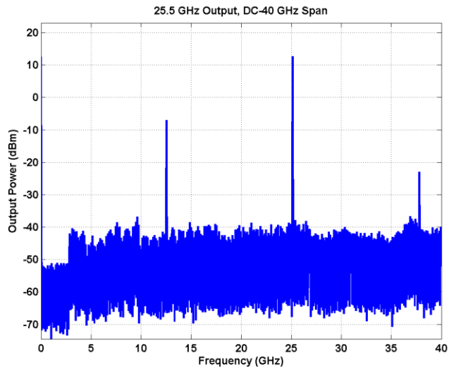
Figure 7 – 25.5 GHz Output, DC-40 GHz, RBW = 1 MHz, VBW = 10 kHz
