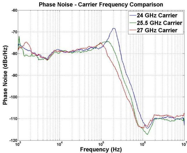
Figure 4 - Representative Phase Noise Plots
