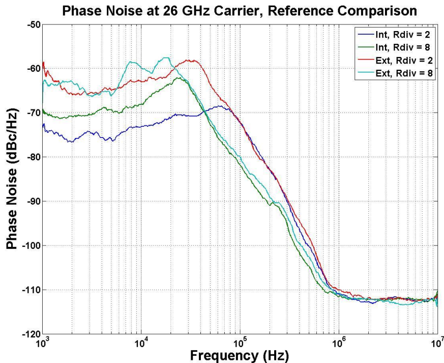
Figure 3 - Phase Noise Reference and Reference Divider Comparison
