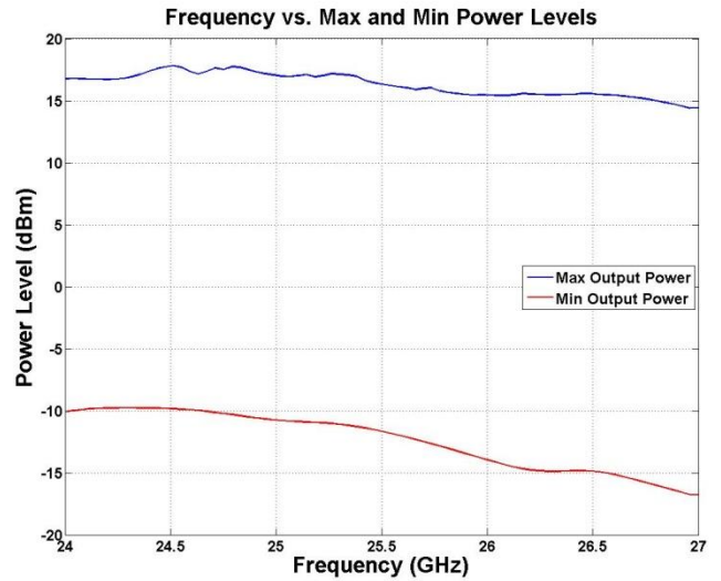
Figure 5 - Frequency vs. Output Power from 24 GHz to 27 GHz in 60 MHz steps
