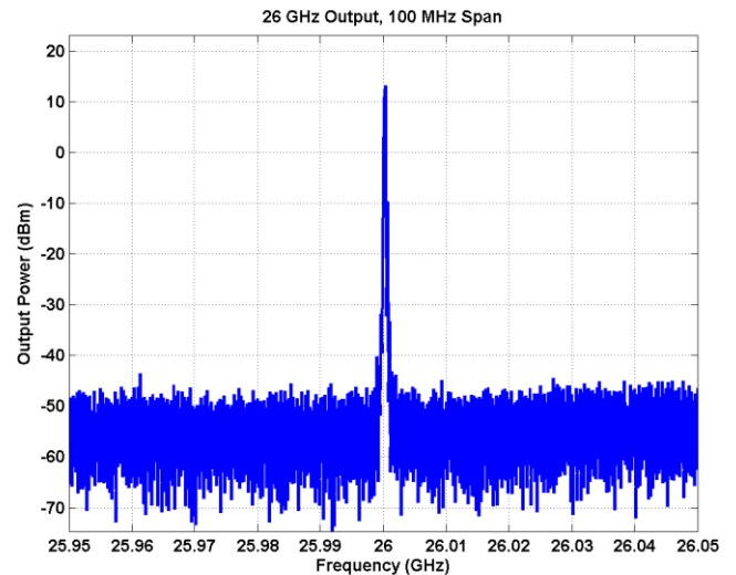
Figure 9 – 26 GHz Output, 100 MHz, RBW = 10 kHz, VBW = 3 kHz
