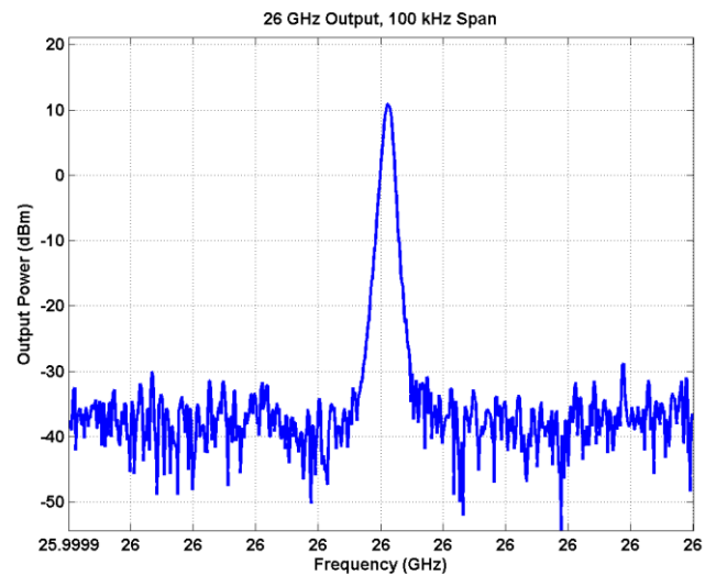
Figure 11 – 26 GHz Output, 100 MHz, RBW = 10 kHz, VBW = 30 Hz
