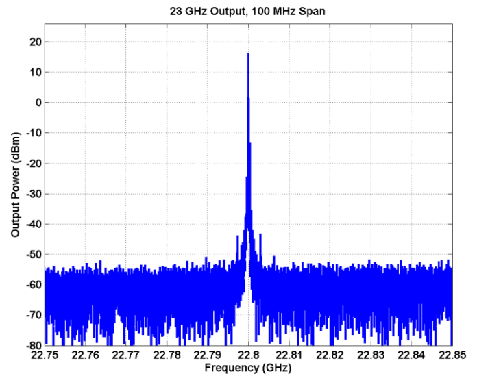
Figure 9 – 23 GHz Output, 100 MHz span, RBW = 10 kHz, VBW = 3 kHz
