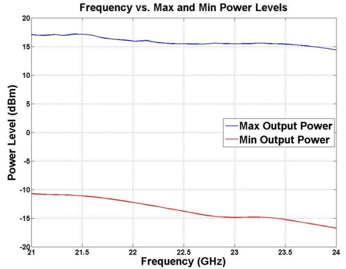
Figure 5 - Frequency vs. Output Power from 21 GHz to 24 GHz in 60 MHz steps
