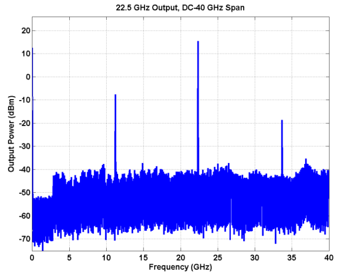
Figure 7 – 22.5 GHz Output, DC-40 GHz, RBW = 1 MHz, VBW = 10 kHz
