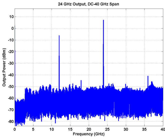
Figure 8 – 24 GHz Output, DC-40 GHz, RBW = 1 MHz, VBW = 10 kHz
