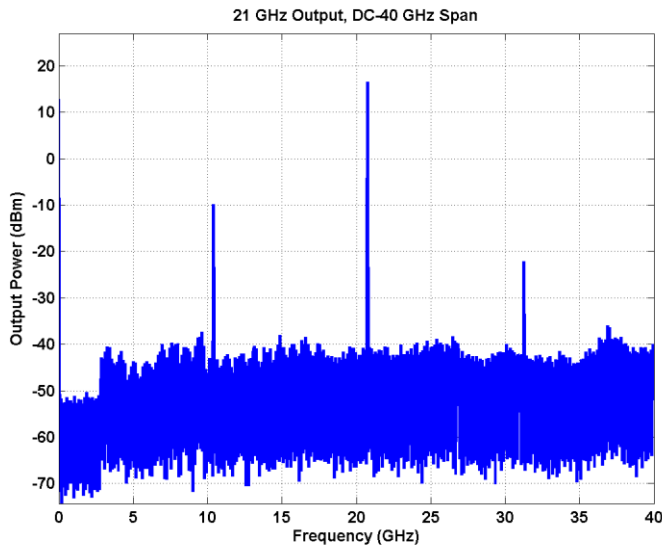
Figure 6 – 21 GHz Output, DC-40 GHz, RBW = 1 MHz, VBW = 10 kHz
