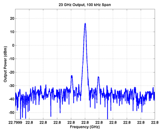
Figure 41 – 23 GHz Output, 100 kHz span, RBW = 100 Hz, VBW = 30 Hz
