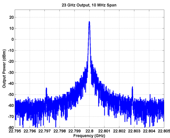
Figure 10 – 23 GHz Output, 10 MHz span, RBW = 3 kHz, VBW = 1 kHz
